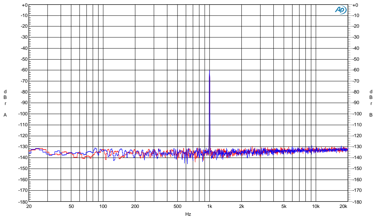
Figure 4. DNR FFT, 1kHz @ -60dB, Single-Ended, 32Ω Load
