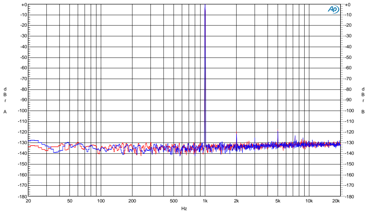
Figure 5. THD+N FFT, 1kHz @ -6dB, Single-Ended, 32Ω Load
