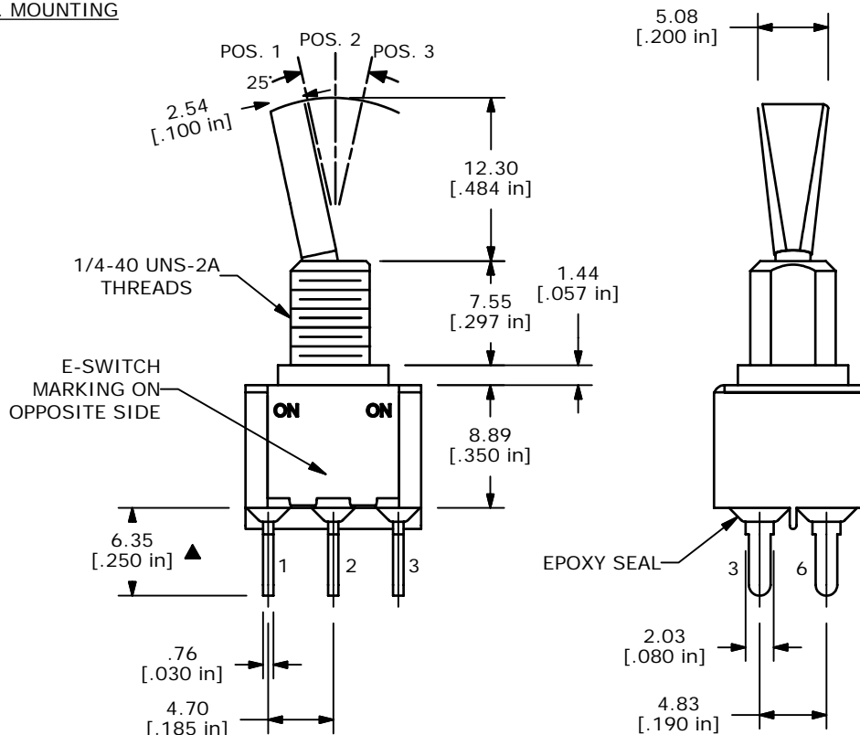
P.C.B. MOUNTING
