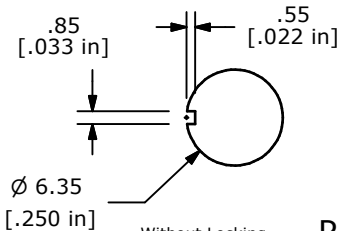
PANEL MOUNTING
