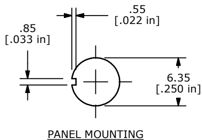
PANEL MOUNTING
