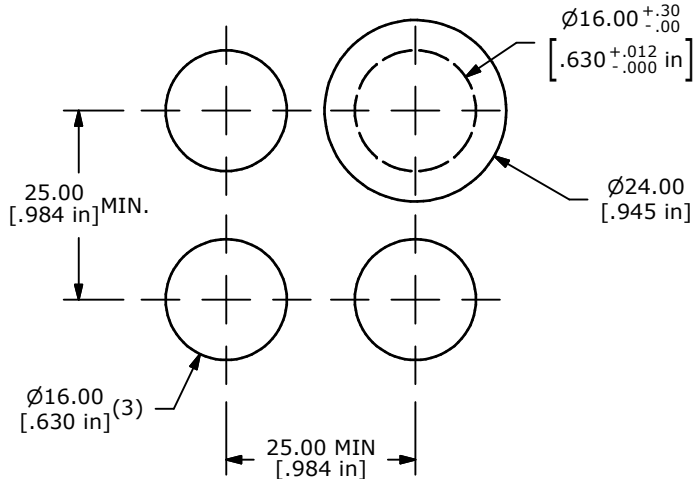
PANEL MOUNTING
