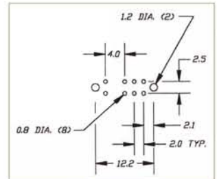
PC MOUNTING
