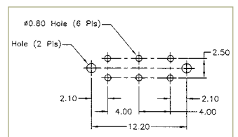
P.C. MOUNTING
