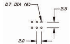
P.C. MOUNTING
