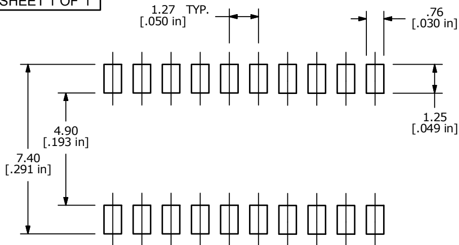
PC LAYOUT
