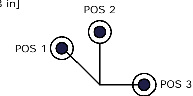
CIRCUIT: SPDT CONTACT CONFIGURATION 45° INDEXING
