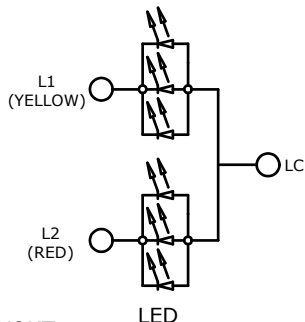
CIRCUIT LAYOUT
