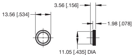
KNURLED NUT WITH COLLAR
