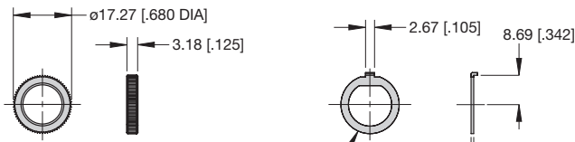
LOCKING RING
