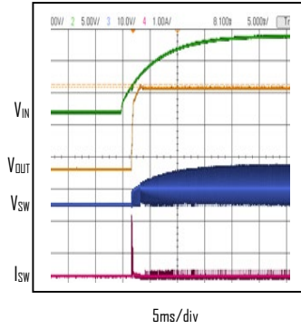
Start-up Waveform with EN=V_IN V_{IN}=12V, V_{OUT}=5V, I_{OUT}=0A
