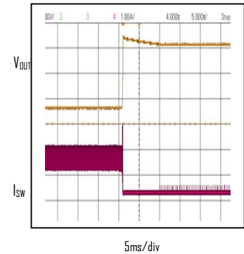
Short-Circuit Recovery V_{IN}=24V, V_{OUT}=5V, I_{OUT}= \text{Short to } 0A
