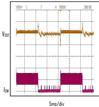
Load Transient Response V_{IN}=12V, V_{OUT}=5V, I_{OUT}=0 \text{ to } 0.5A
