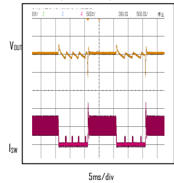
Load Transient Response V_{IN}=12V, V_{OUT}=3.3V, I_{OUT}=0 \text{ to } 0.5A
