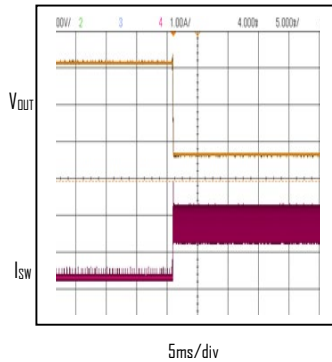
Short-Circuit Response V_{IN}=24V, V_{OUT}=5V, I_{OUT}=0A \text{ to Short}
