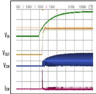
Start-up Waveform with EN= V_{IN} V_{IN}=12\text{V}, V_{OUT}=5\text{V}, I_{OUT}=0\text{A}
