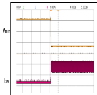
Short-Circuit Response V_{IN}=24\text{V}, V_{OUT}=5\text{V}, I_{OUT}=0\text{A} to Short
