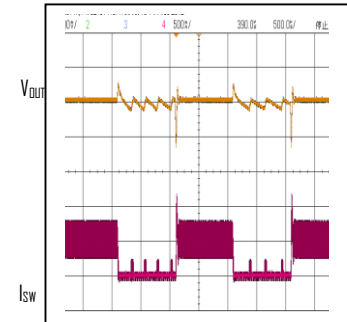
Load Transient Response V_{IN}=12\text{V}, V_{OUT}=3.3\text{V}, I_{OUT}=0 to 0.5\text{A}
