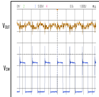
Switching Waveform V_{IN}=12\text{V}, V_{OUT}=5\text{V}, I_{OUT}=0.3\text{A}
