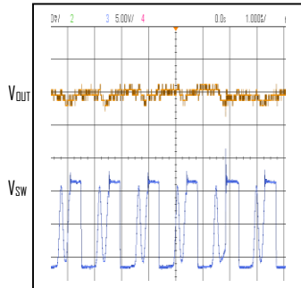
Switching Waveform V_{IN}=12\text{V}, V_{OUT}=5\text{V}, I_{OUT}=0.1\text{A}
