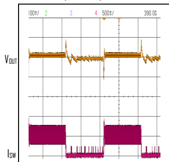
Load Transient Response V_{IN}=12\text{V}, V_{OUT}=5\text{V}, I_{OUT}=0 to 0.5\text{A}
