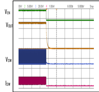
Shutdown Waveform with EN V_{IN}=30\text{V}, V_{OUT}=5\text{V}, I_{OUT}=0.5\text{A}
