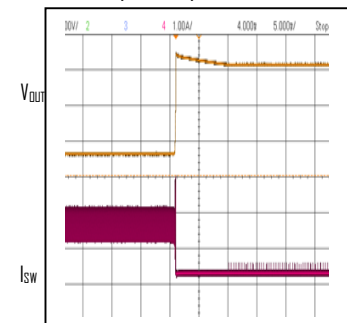
Short-Circuit Recovery V_{IN}=24\text{V}, V_{OUT}=5\text{V}, I_{OUT}=\text{Short} to 0\text{A}
