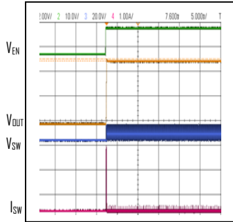
Start-up Waveform with EN V_{IN}=12\text{V}, V_{OUT}=5\text{V}, I_{OUT}=0\text{A}
