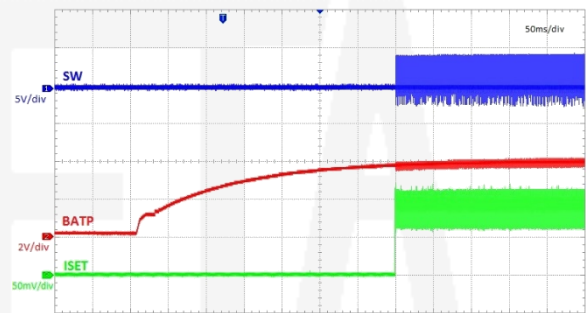
V TOP plug-in Start-Up , V BOOT = Shorted , R SET = 50k, V TOP = 4.3V
