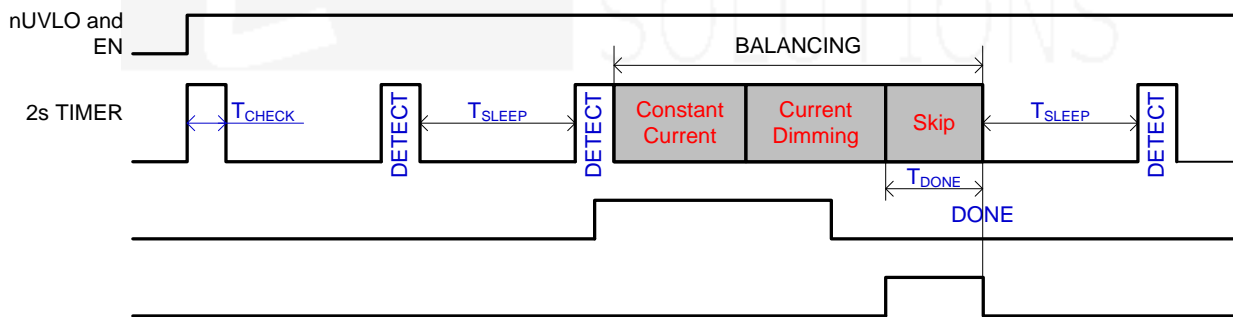
Figure 4: Timing Profile
