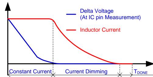
Figure 5: Balancing Profile
