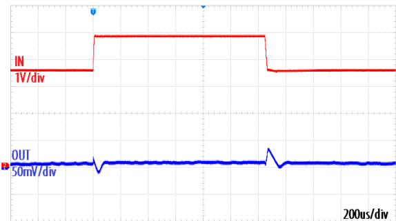
Load Regulation, V_{IN}=5\text{V} , V_{OUT}=3.3\text{V}
