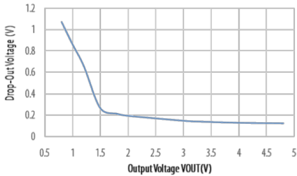
Drop-out Voltage vs. Output Voltage, I_{OUT}=1\text{A}
