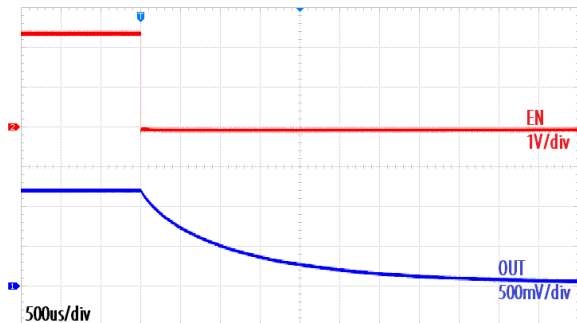
Shutdown Waveform at No Load, V_{OUT}=1.2\text{V}
