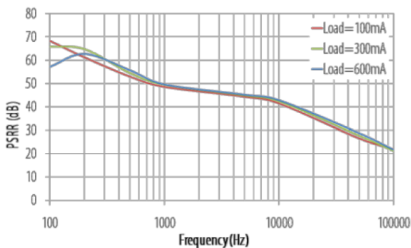
Power Supply Rejection vs. Output Current V_{OUT}=1.8\text{V} , C_{IN}=C_{OUT}=10\mu\text{F}
