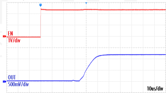
Start-Up Waveform with R_{OUT} = 1.2\Omega , V_{OUT}=1.2\text{V}
