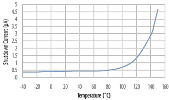
Shutdown Current over Temperature
