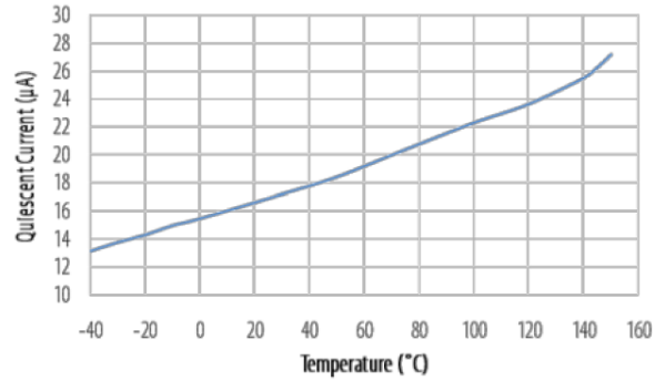
Quiescent Current over Temperature
