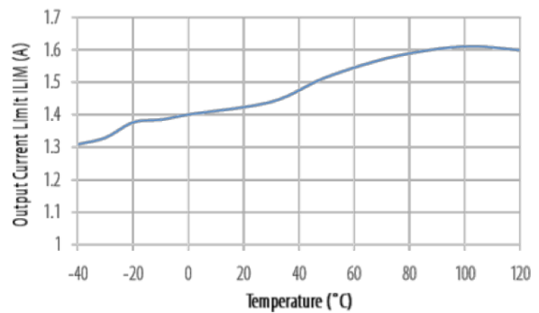
Current Limit vs. Temperature
