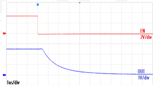
Shutdown Waveform with R_{OUT} = 2.5\Omega , V_{OUT}=2.5\text{V}
