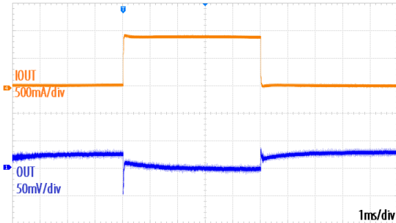
Line Transient, V_{IN}=3.9\text{V} - 5\text{V} , I_{OUT}=1\text{mA} , V_{OUT}=3.3\text{V}
