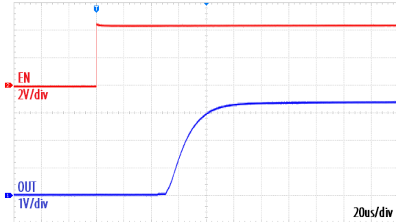
Start-Up Waveform at No Load, V_{OUT}=3.3\text{V}
