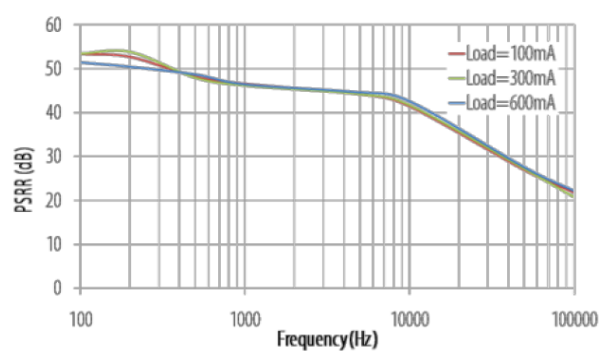
PSRR vs. Frequency and Output Current, V_{OUT}=3.3\text{V} , C_{IN}=C_{OUT}=10\mu\text{F}
