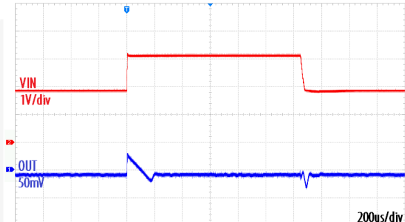
Line Regulation, V_{IN}=5\text{V} , V_{OUT}=3.3\text{V}
