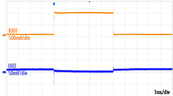
Line Transient, V_{IN}=2.2\text{V} - 3.2\text{V} , I_{OUT}=1\text{mA} , V_{OUT}=1.2\text{V}
