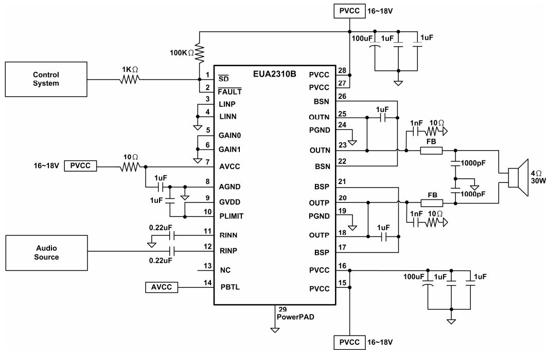
Figure 42. 4Ω/30W PBTL Output
