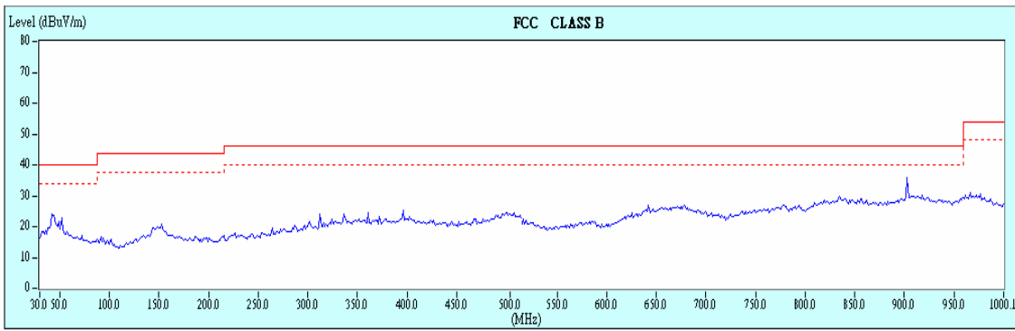
Figure39. EMI Test and FCC Limits
