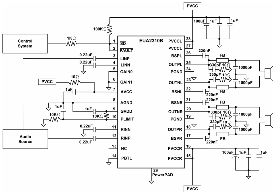
Figure 41. Single Ended Input
