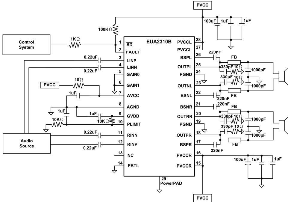
Figure 40. Differential Input
