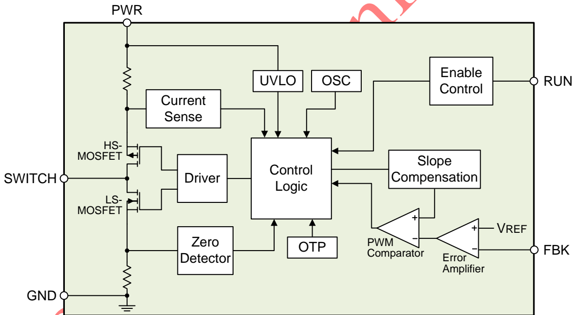
Figure 1. EA8103 internal function block diagram
