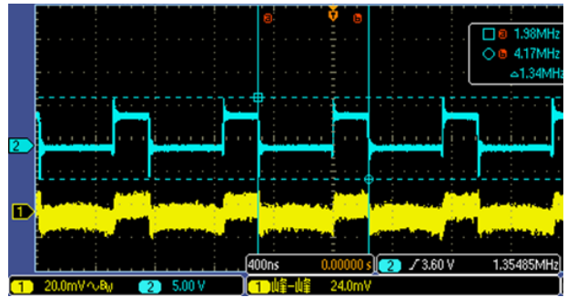
VIN = 5V, ILOAD = 1.2A Waveform
