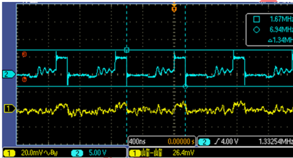
VIN = 5V, ILOAD = 0.1A Waveform
