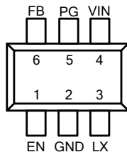
Figure 1. Pin Assignment of EA8107
