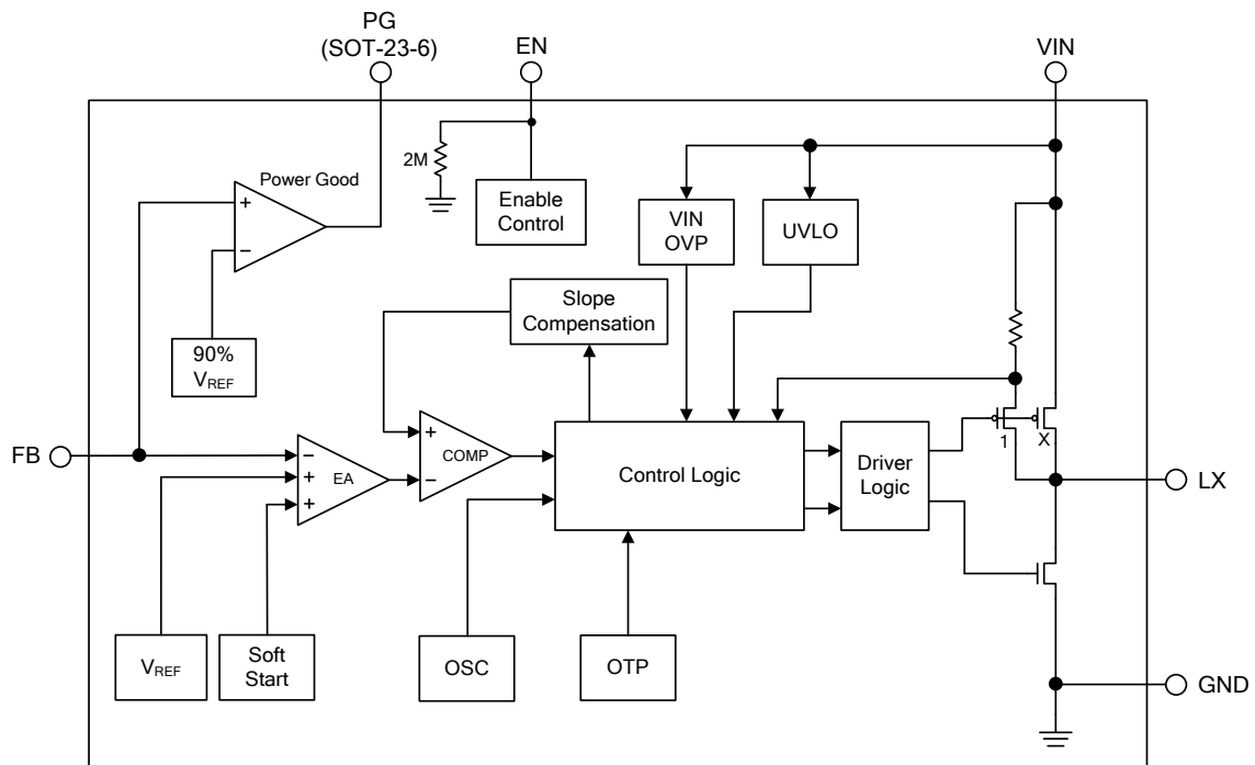
Figure 3. Block Diagram of EA8107
