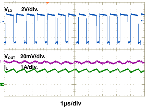
Figure 7. Steady State Waveform
