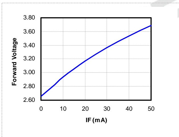
3. Relative Forward Voltage vs. Forward Current (T S =25 °C)
