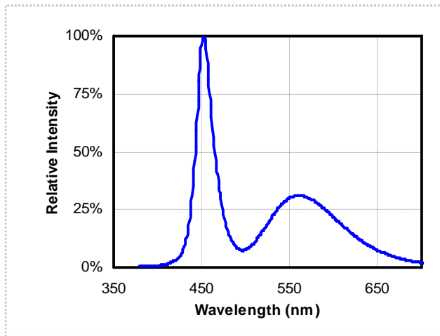
1. Spectrum Distribution (T S =25 °C, I F =20mA)
