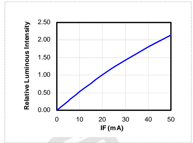
2. Relative Luminous Flux vs. Forward Current (T S =25 °C)
