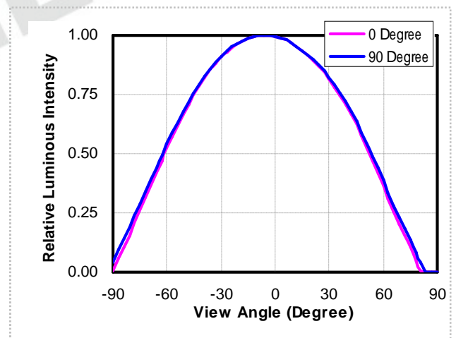
4. Radiation Diagram (T S =25 °C, I F =20mA)
