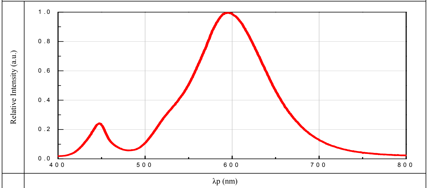
Relative Spectral Distribution , I_F=1000\text{mA} @ 50\text{ms} , T_{\text{solder pad}}=25^\circ\text{C}
