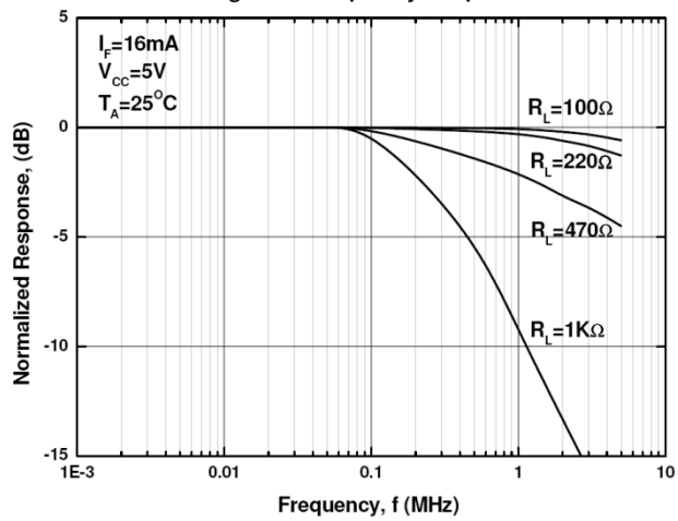
Figure 8. Frequency Response
