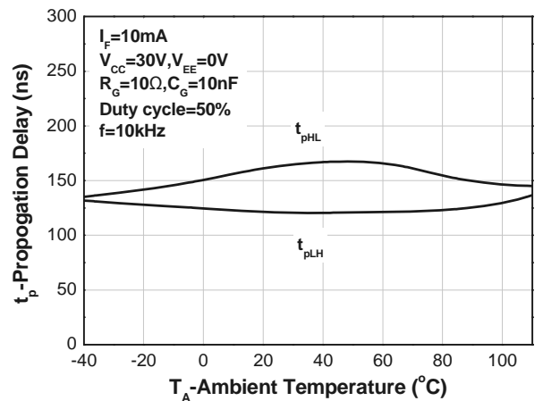
Fig.12 Propagation Delay vs. Ambient Temperature
