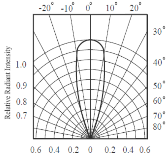
Fig.6 Relative Radiant Intensity vs. Angular Displacement
