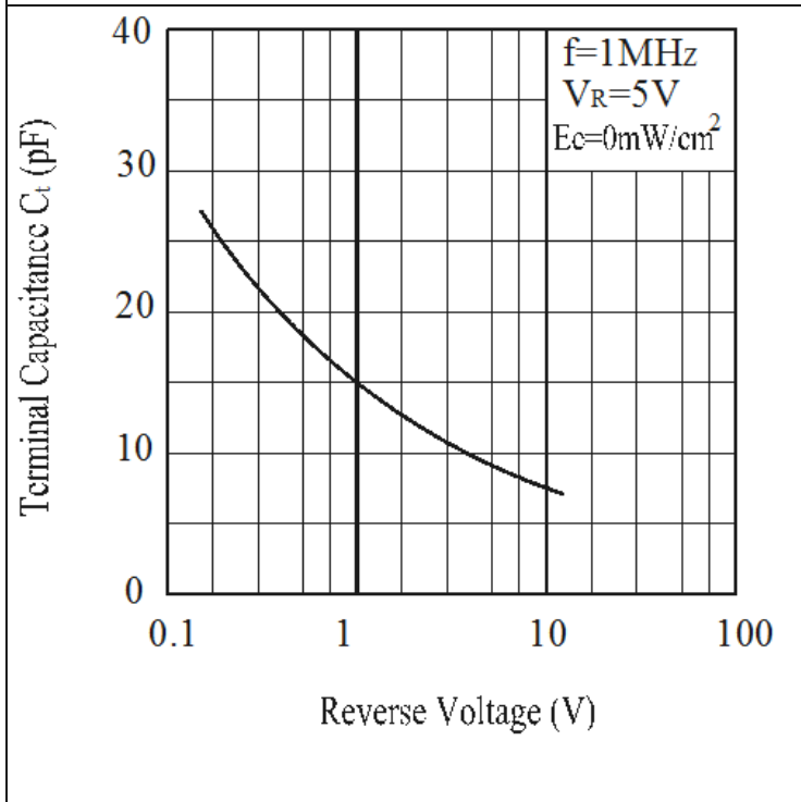
Terminal Capacitance vs. Reverse Voltage
