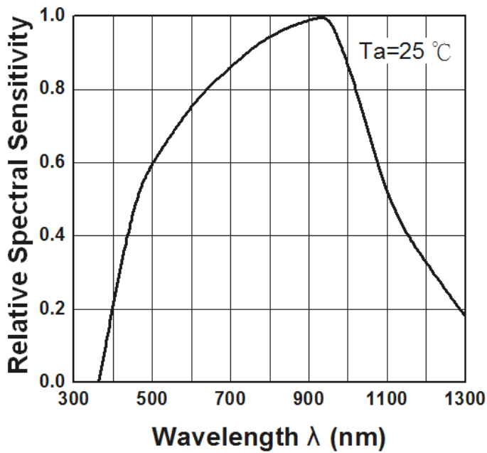
Fig.1 Spectral Sensitivity
