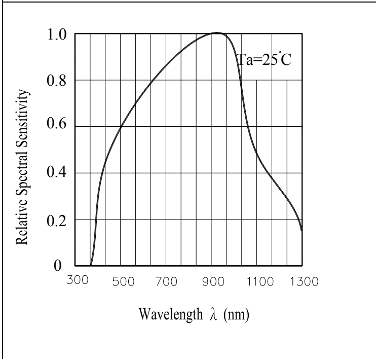
Spectral Sensitivity
