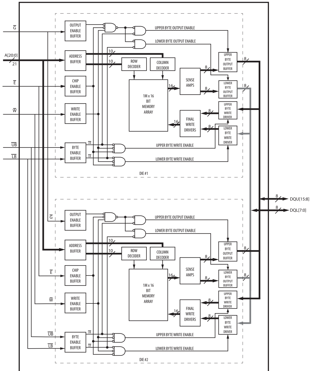
Figure 1.1 Block Diagram
