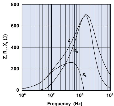
Figure 9A Impedance, reactance, and resistance vs. frequency for chip bead 2506036017Y0.
