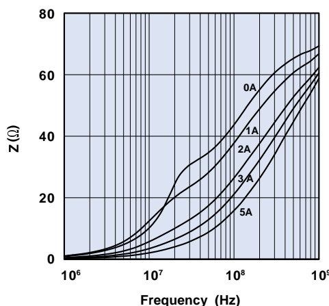
Figure 9B Impedance vs. frequency with dc bias as parameter for SM bead 2761019447.
