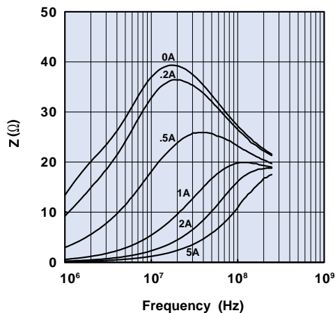
Figure 7B Impedance vs. frequency with dc bias as parameter for SM bead 2773019447.
