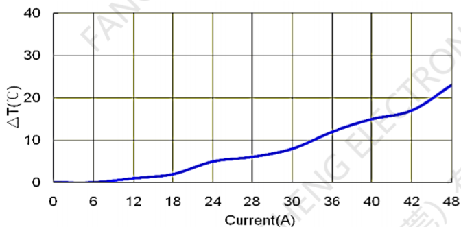
Current VS Temperature
