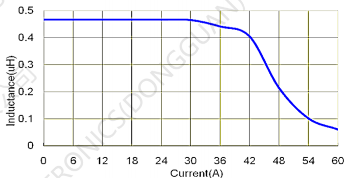
Inductance VS Current
