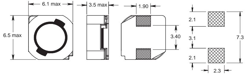
Recommended layout for solder pads
