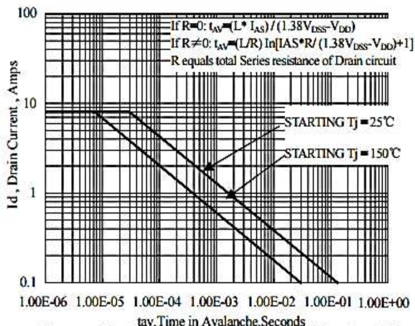
Figure 16 Unclamped Inductive Switching Capability
