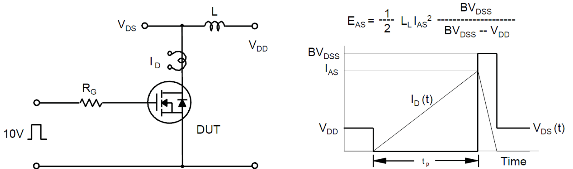
Fig 19. Unclamped Inductive Switching Test Circuit & Waveforms
