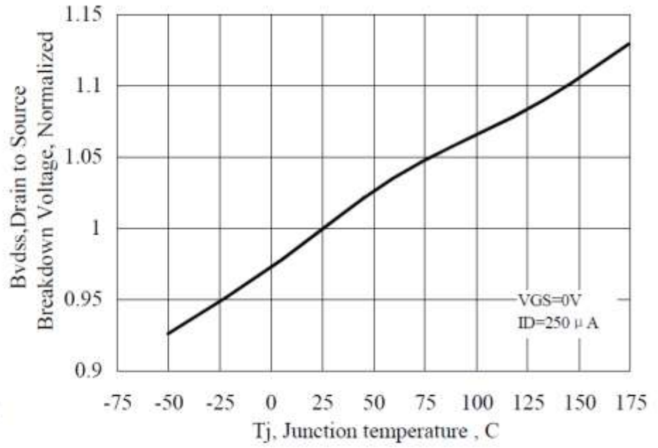
Figure 12 Typical Breakdown Voltage vs Junction Temperature
