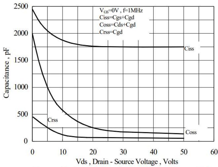
Figure 13 Typical Capacitance vs Drain to Source Voltage
