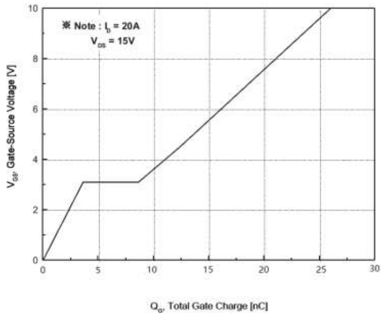
Fig.7 Gate Charge Characteristics
