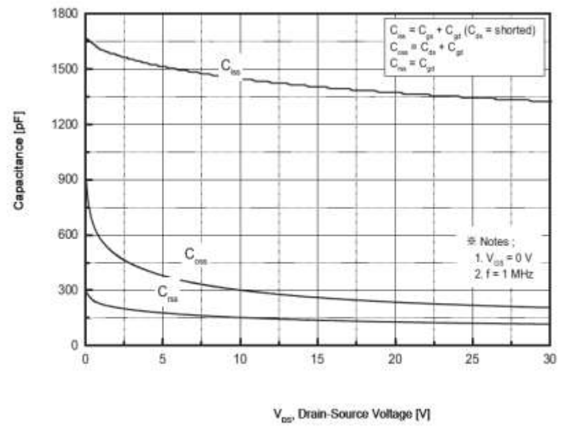
Fig.8 Capacitance Characteristics
