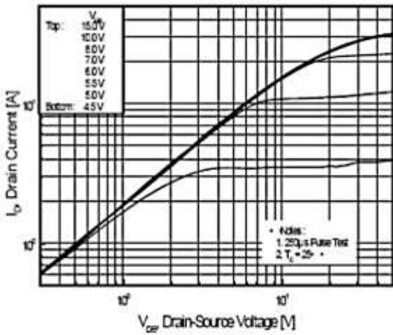
Figure 1. On-Region Characteristics
