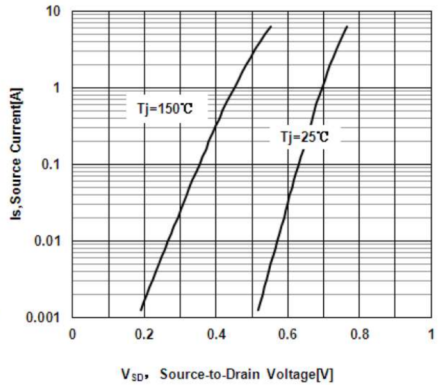
Figure 7 Typical Body Diode Transfer Characteristics
