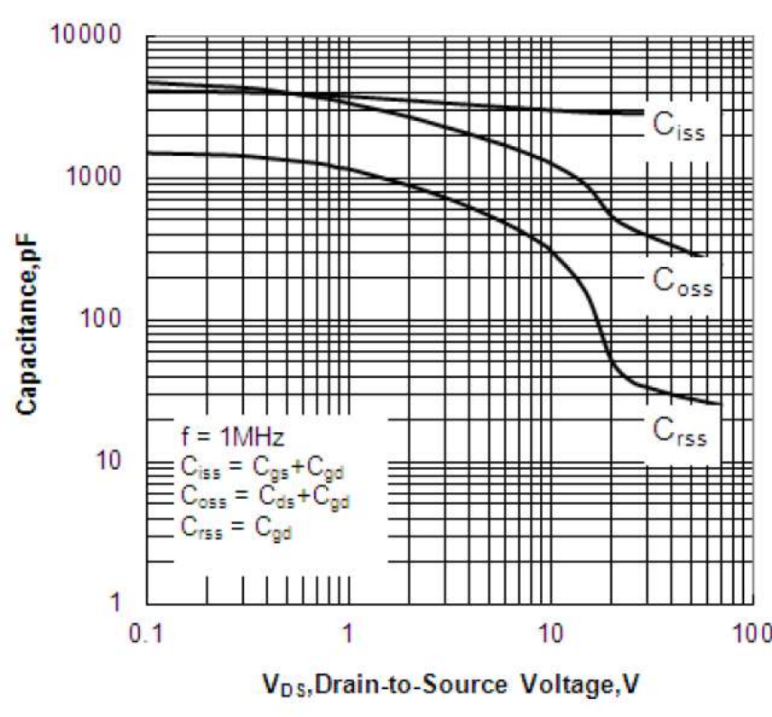
Figure 12 Typical Capacitance vs Drain to Source Voltage
