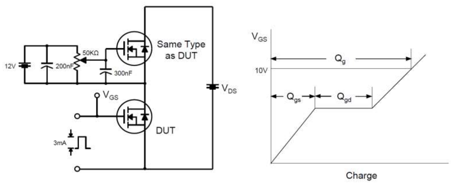
Fig 14. Gate Charge Test Circuit & Waveform
