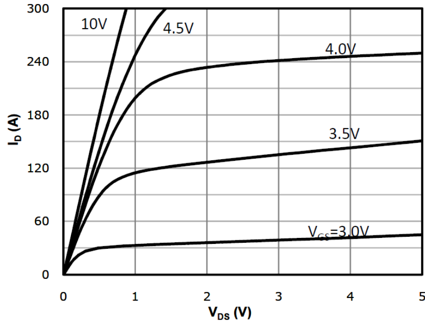
Fig 1: Output Characteristics
