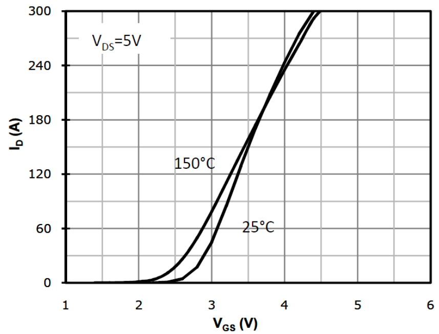
Fig 2: Transfer Characteristics
