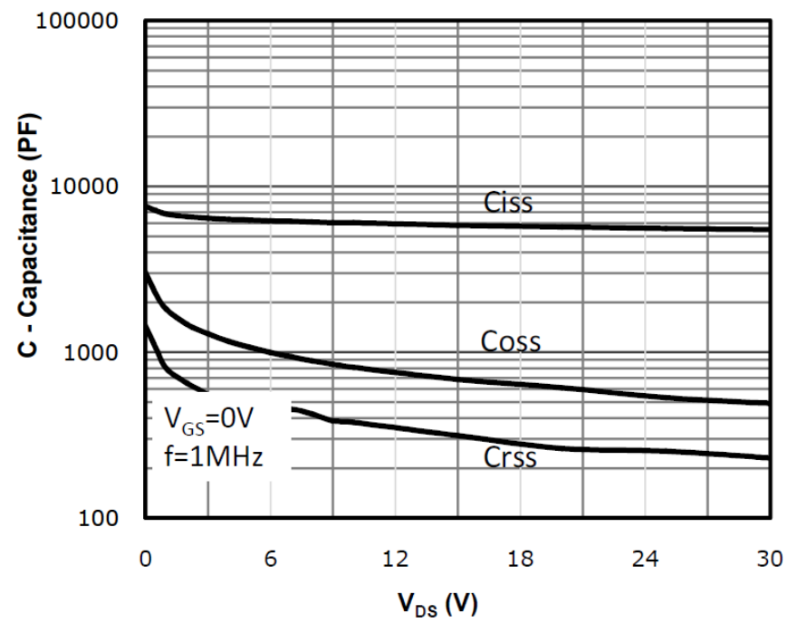
Fig 6: Capacitance Characteristics
