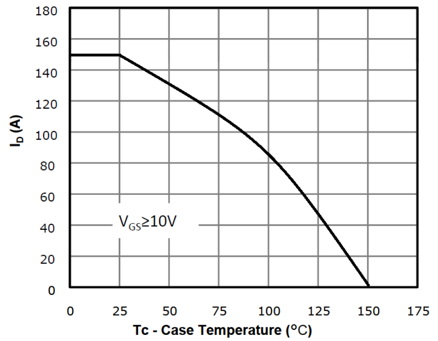
Fig 10: Drain Current Derating
