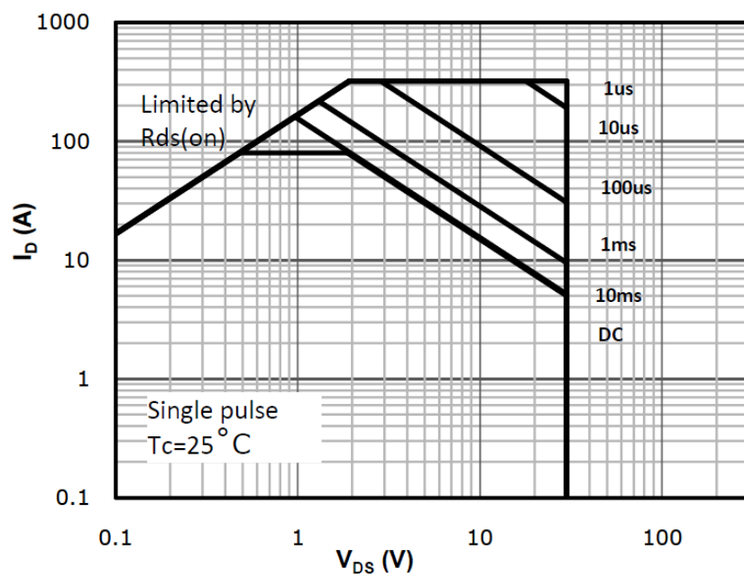
Fig 11: Safe Operating Area
