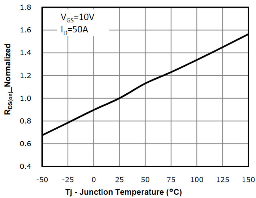
Fig 5: R_{DS(on)} vs. Temperature
