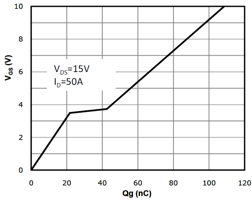
Fig 7: Gate Charge Characteristics
