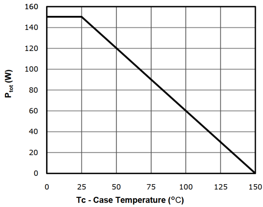
Fig 9: Power Dissipation
