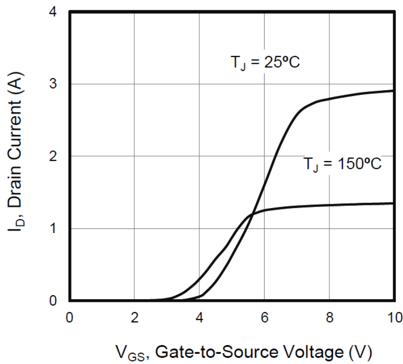
Figure 5. Transfer Characteristics
