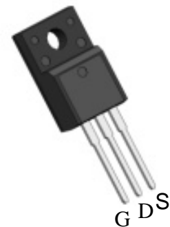
TO-220F FHF series
