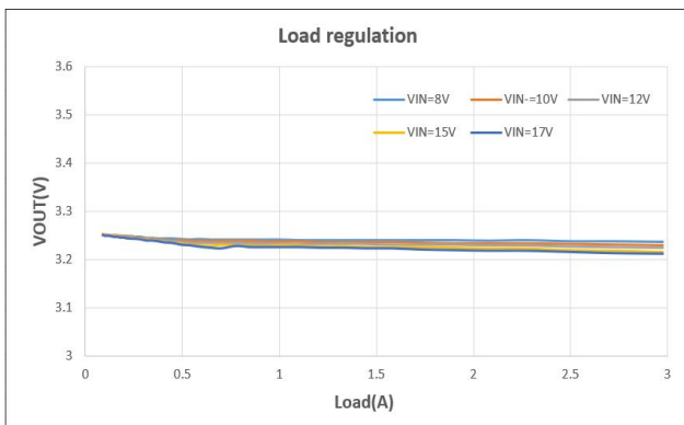
负载调整率 ( V_{OUT} = 3.25V )
