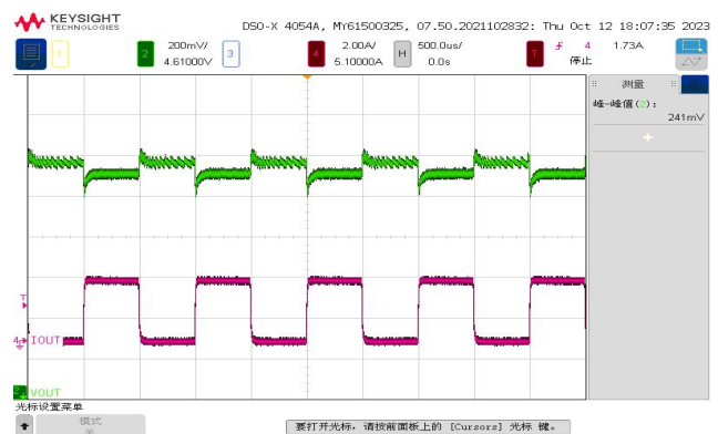
负载动态响应, V_{OUT} = 5V , I_{OUT} = 0A \rightarrow 3A
