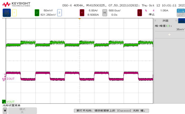
负载动态响应, V_{OUT} = 1V , I_{OUT} = 0A \rightarrow 3A
