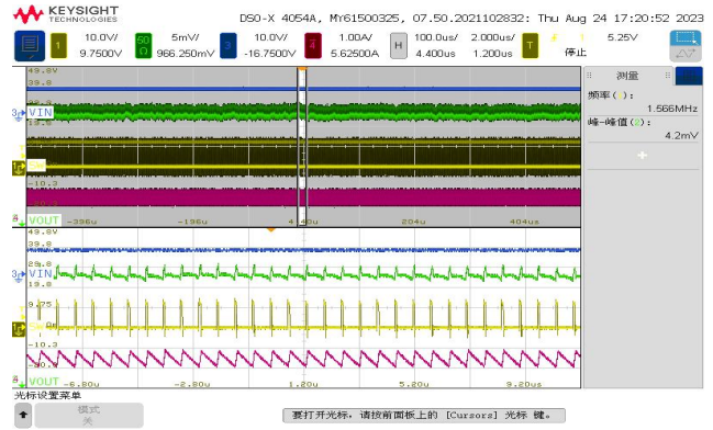
稳态, V_{IN} = 12V , V_{OUT} = 1.0V I_{OUT} = 3A
