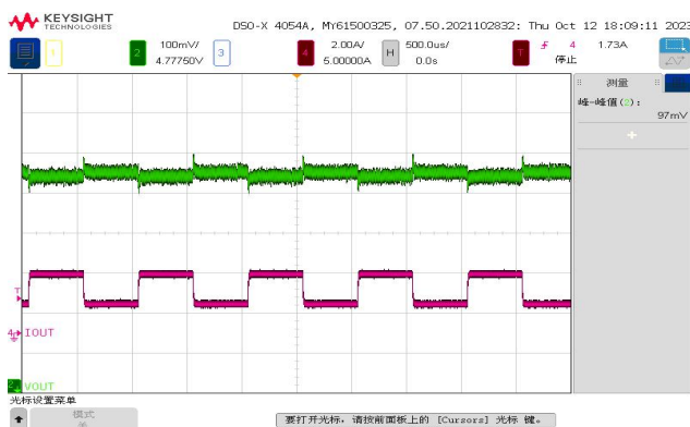
负载动态响应, V_{OUT} = 5V , I_{OUT} = 1.5A \rightarrow 3A
