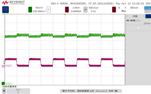
负载动态响应, V_{OUT} = 1V , I_{OUT} = 0A \rightarrow 1.5A
