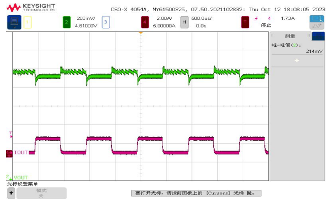
负载动态响应, V_{OUT} = 5V , I_{OUT} = 0A \rightarrow 1.5A
