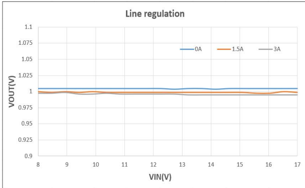
线性调整率 ( V_{OUT} = 1.0V )
