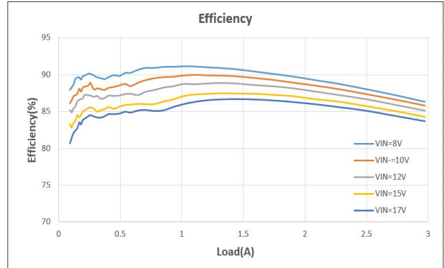
输出电流 vs 效率 ( V_{OUT} = 3.25V )
