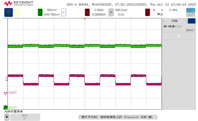
负载动态响应, V_{OUT} = 1V , I_{OUT} = 1.5A \rightarrow 3A
