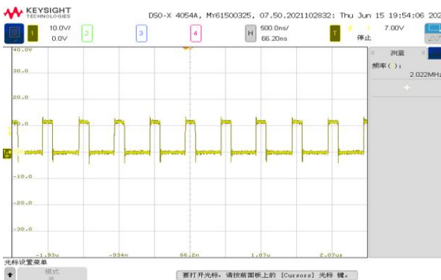
开关频率 V_{OUT} = 3.3V , I_{OUT} = 3A
