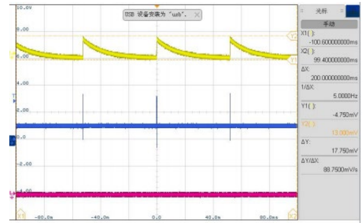
输出纹波, V_o = 1.0V, I_o = 6A
