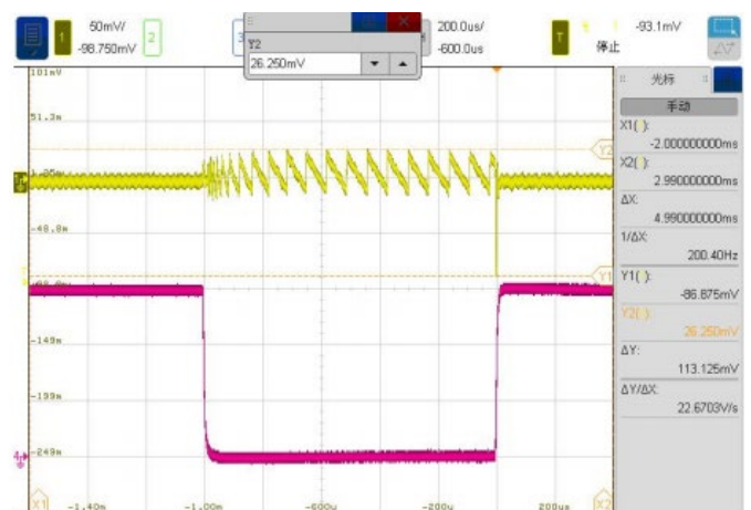
负载动态响应, V_{OUT} = 0.8V, I_{OUT} = 0A \rightarrow 6A
