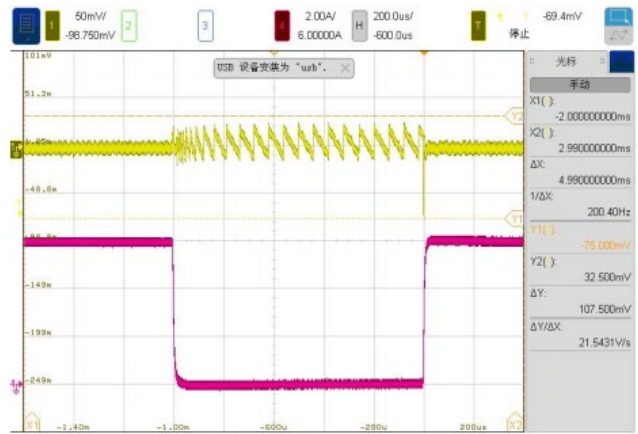
负载动态响应, V_{OUT} = 1.0V, I_{OUT} = 0A \rightarrow 6A
