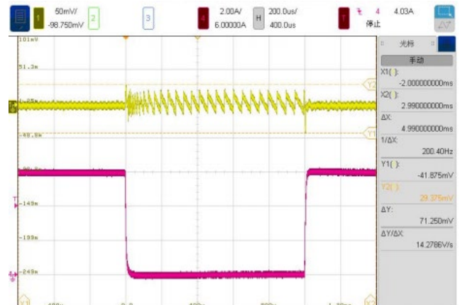
负载动态响应, V_{OUT} = 1.8V, I_{OUT} = 0A \rightarrow 6A
