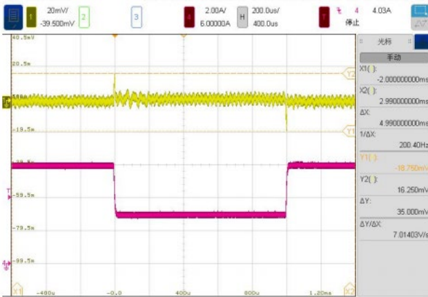
负载动态响应, V_{OUT} = 1.8V, I_{OUT} = 3A \rightarrow 6A
