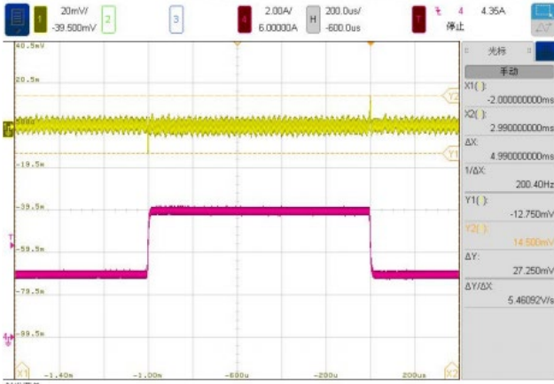
负载动态响应, V_{OUT} = 1.0V, I_{OUT} = 3A \rightarrow 6A
