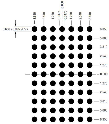
TOP VIEW (PCB LAYOUT 建议尺寸)
