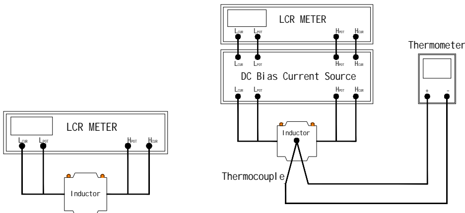
Is & RDC test schematic diagram Isat & Irms test schematic diagram
