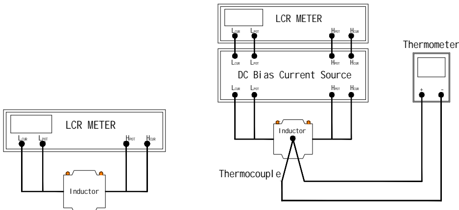
Ls & RDC test schematic diagram
