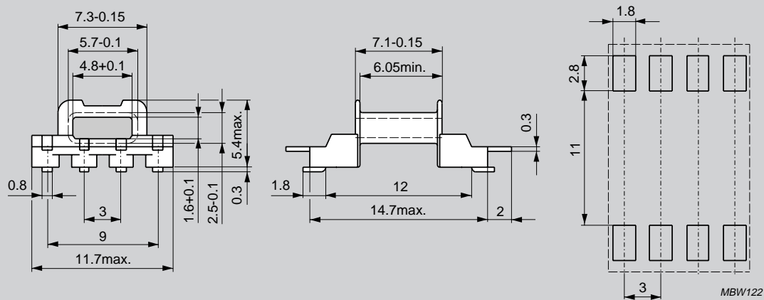
Fig. 1 SMD coil former for EFD10
