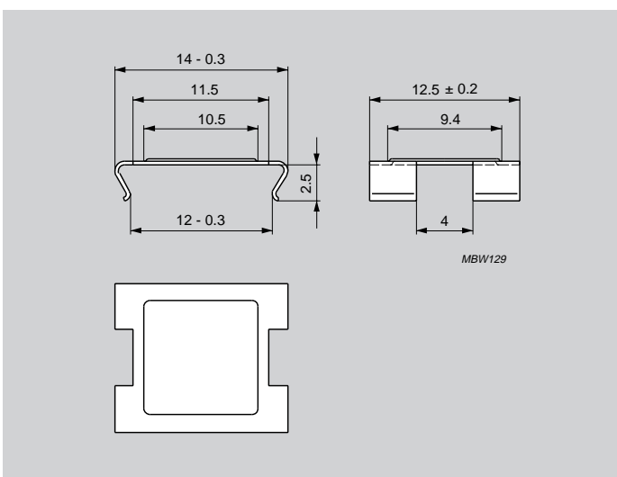
Fig. 2 clamp for EFD12
