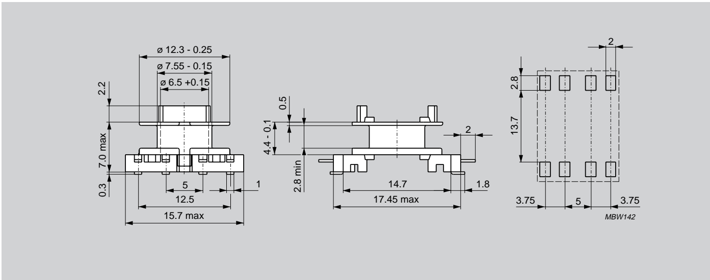
Fig. 1 SMD coil former for RM6S/ILP
