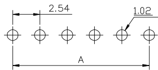
PCB LAYOUT
