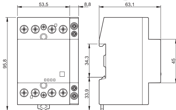
Type 022.63 / 022.65 Screw terminal
