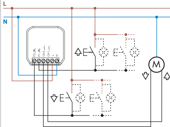
Maximum 5 ( \leq 1 mA) illuminated push buttons
