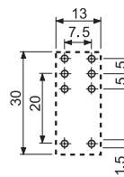
95.15.2 Copper side view
