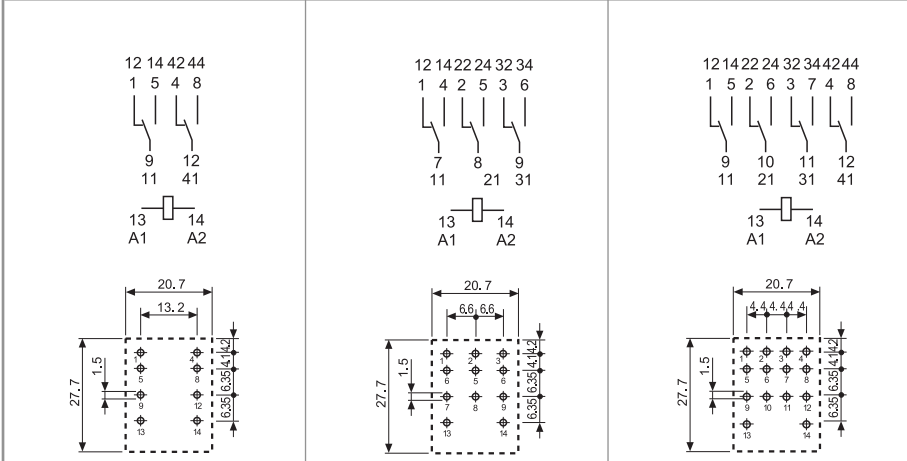
Copper side view Copper side view Copper side view
