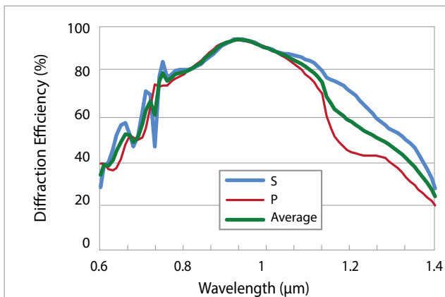
Typical absolute diffraction efficiency at AOI 44.2° *
